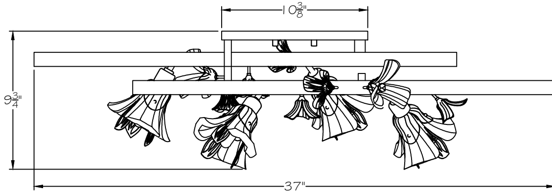
TOP VIEW
